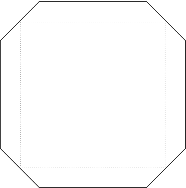
2.5" square Cut 3.204" Face 2.5" Bleed 0.352" flats 0.0219" corners
