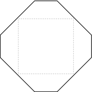
1" square Cut 1.652" Face 1" Bleed 0.326" flats 0.0212" corners
