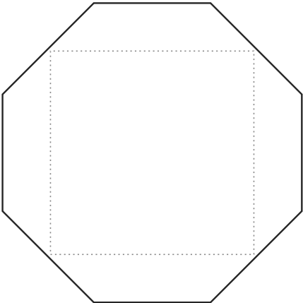
1.5" square Cut 2.207" Face 1.5" Bleed 0.3535" flats 0.024" corners
