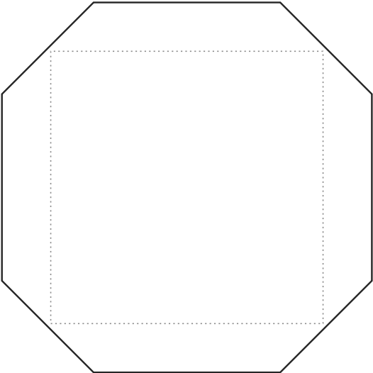
2" square Cut 2.717" Face 2" Bleed 0.3585" flats 0.0311" corners
