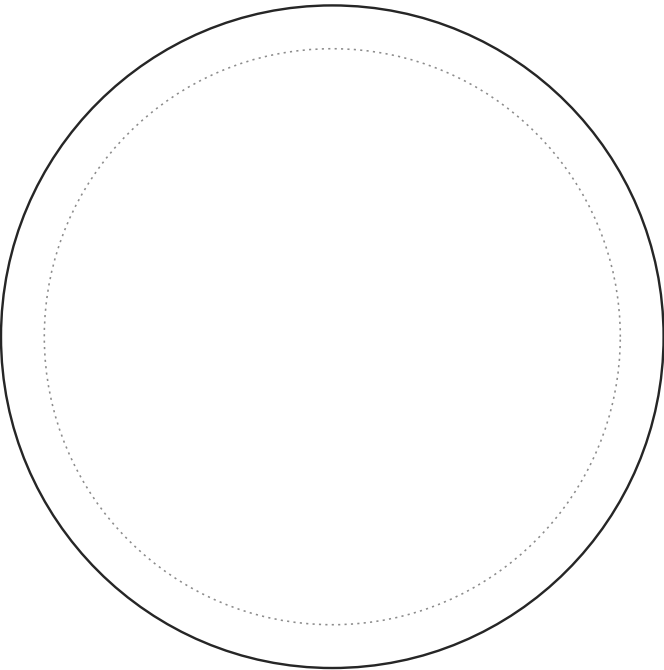
3" round Cut 3.451" Face 3" Bleed 0.2255" per side
