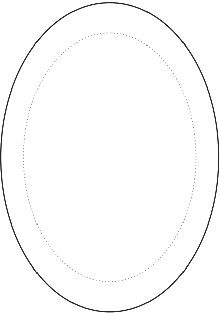
45 x 65mm oval Cut 57 x 81mm Face 45 x 65mm Bleed 6mm sides 8mm ends
