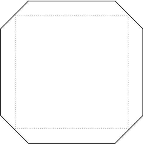
50mm square Cut 63mm Face 50mm Bleed 6.5mm flats 0.51mm corners
