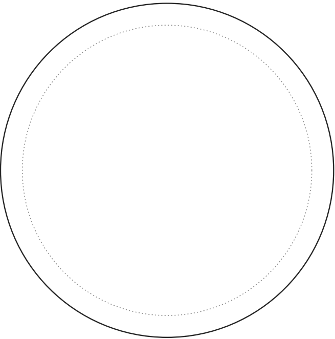
75mm round Cut 86.3mm Face 75mm Bleed 5.65mm per side
