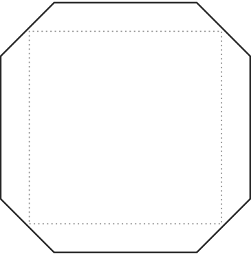
37mm square Cut 48mm Face 37mm Bleed 5.5mm flats 0.51mm corners
